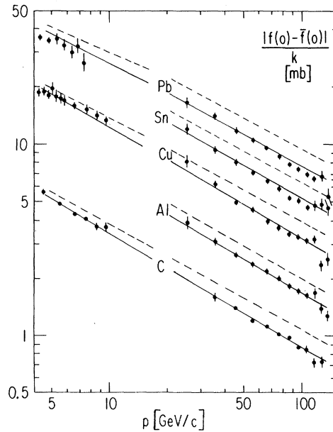
FIG. 3. |f - \bar{f}|/k data with optical-model predictions, including inelastic screening. The data are the same as in Fig. 2. Dashed lines are predictions using elementary inputs, i.e., \alpha_\omega(0) = 0.44 ; full lines use the effective intercept " \alpha_\omega(0) = 0.39 ".
